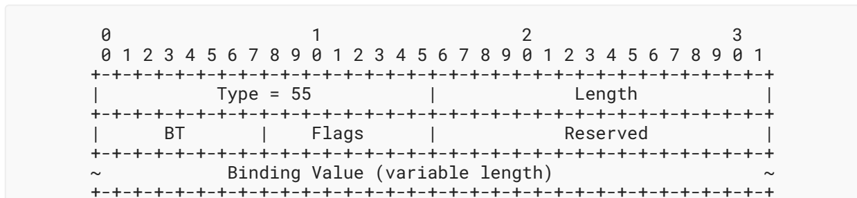
Figure 2: TE-PATH-BINDING TLV
